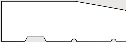
PROFILE 913 140mm x 45mm
