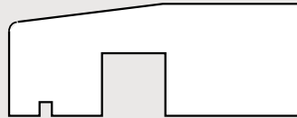
PROFILE 912 95mm x 36mm
